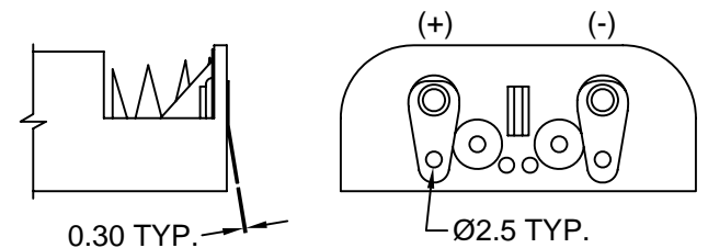
PDSN-14C SOLDER LUGS
