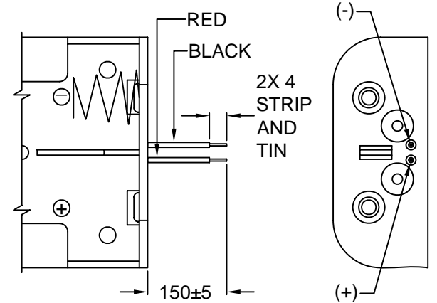
PDSN-14A WIRE LEADS
